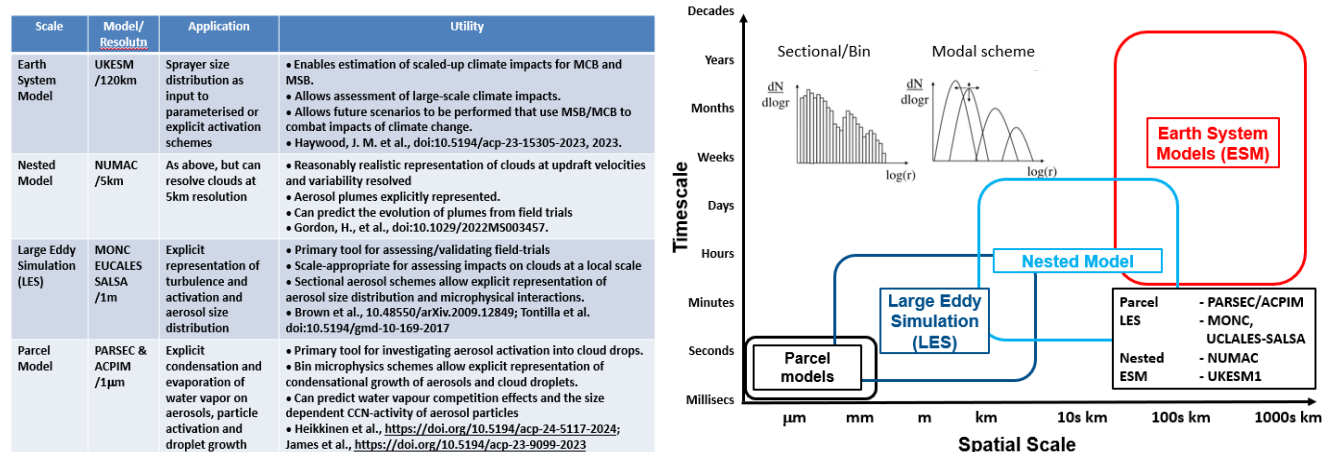
Figure 2. Left Panel): details of the specific models that are proposed. Right Panel): models and their spatial scales and schematic of sectional and modal aerosol size distributions.
