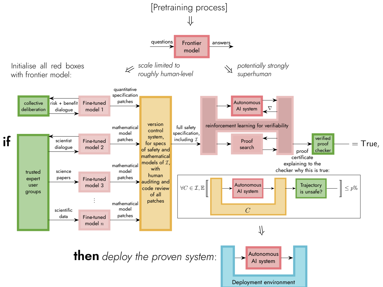
Figure 1: The “gatekeeper” approach can be seen as a scalable general-purpose workflow which consumes general-purpose frontier AI base models and produces safe AI systems specialised to particular tasks with well-defined contexts of use.
