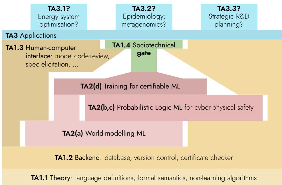
Figure 4: The interfaces between all technical subareas can be shown visually as horizontal contacts.
